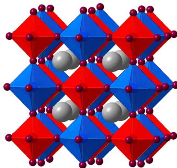
Figure 1. The A_2MM'O_6 double perovskite structure. The large A cations are shown in gray, while the M and M' centered octahedra are shown in red and blue, respectively.
