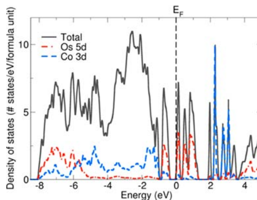
Figure 6. Total- and atom-resolved density of states of \text{Sr}_2\text{CoOsO}_6 from a noncollinear DFT calculation with U_{\text{Co}} = 4.1 eV and U_{\text{Os}} = 2.1 eV. The contributions of the Os 5d and Co 3d orbitals are shown in red and blue, respectively.
