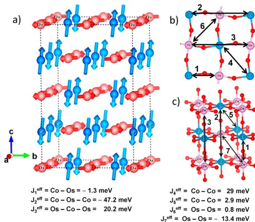
Figure 8. (a) Experimentally determined magnetic structure of Sr 2 CoOsO 6 , with the Os shown in red and the Co in blue. (b) A schematic of the superexchange pathways between Co and Os ions with the exchange constants extracted from the DFT calculations. A positive (negative) value of J indicates ferromagnetic (antiferromagnetic) coupling.
